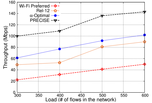
Fig. 8: Throughput for different load.
