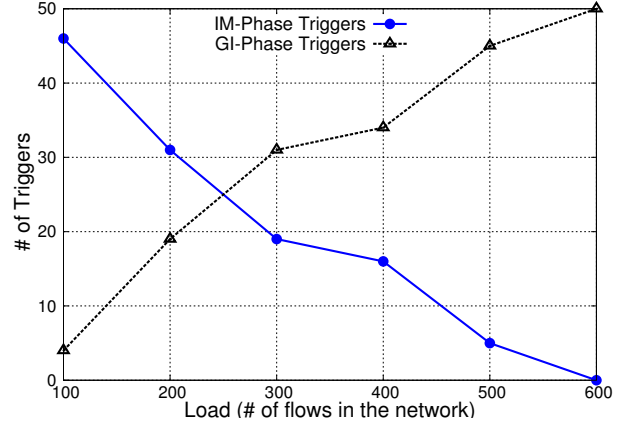
Fig. 6: Triggers for different threshold.
