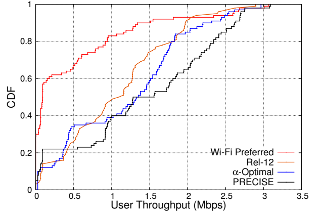
Fig. 7: CDF of UEs throughput.
