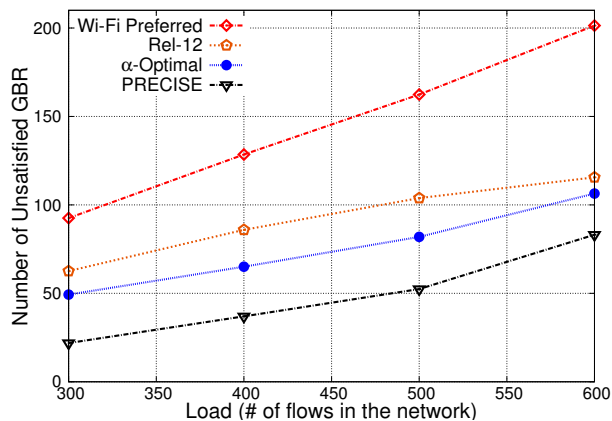
Fig. 9: Unsatisfied GBR.
